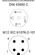
Connector Pin Layout
